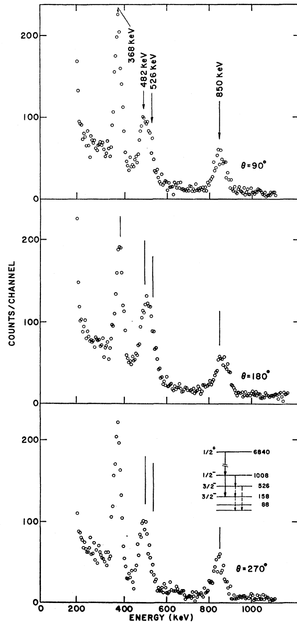
FIG. 5. Examples of the spectra in coincidence with gamma rays of about 5.83 MeV. These were used to determine the spin of the level at 1.008 MeV in \text{Ni}^{88} . For comments about the level scheme, see the caption for Fig. 4. An analysis of the line at 850 keV was used to determine the spin of the level at 1.008 MeV.
