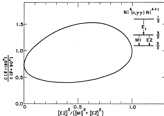
FIG. 1. The computed anisotropy as a function of the multipole mixture for a typical case. Effects of the size, shape, and relative positions of the sample and crystals have been neglected.
