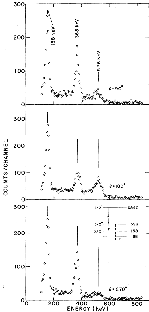
FIG. 4. Examples of the spectra in coincidence with gamma rays of about 6.31 MeV. These were used to determine the spin of the level at 0.526 MeV in \text{Ni}^{88} . The level scheme is based on the work of Fulmer and McCarthy (Ref. 2). The solid lines indicate the cascade that was studied to determine the spin. The dashed lines indicate the origin of the other lines that appear in the spectrum. It should be noted that it was the intensity of the line at 368 keV that was analyzed in this case and not the transition (526 keV) to the ground state.
